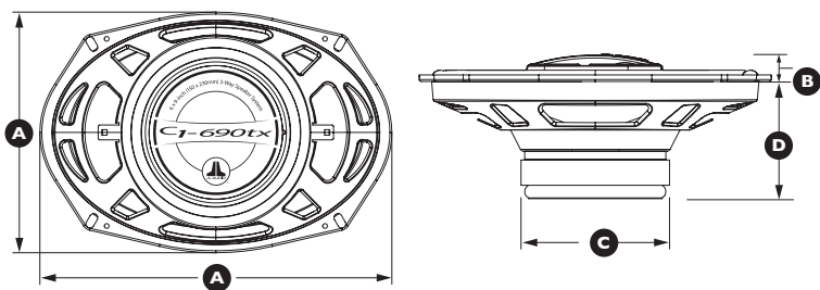
Coaxial Physical Dimensions
