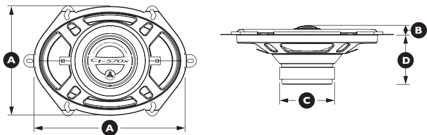
Coaxial Physical Dimensions
