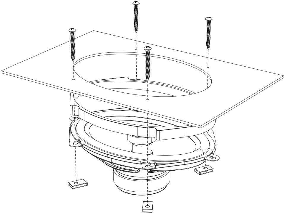
DIAGRAM A: Speaker Installation with Spacer Ring
