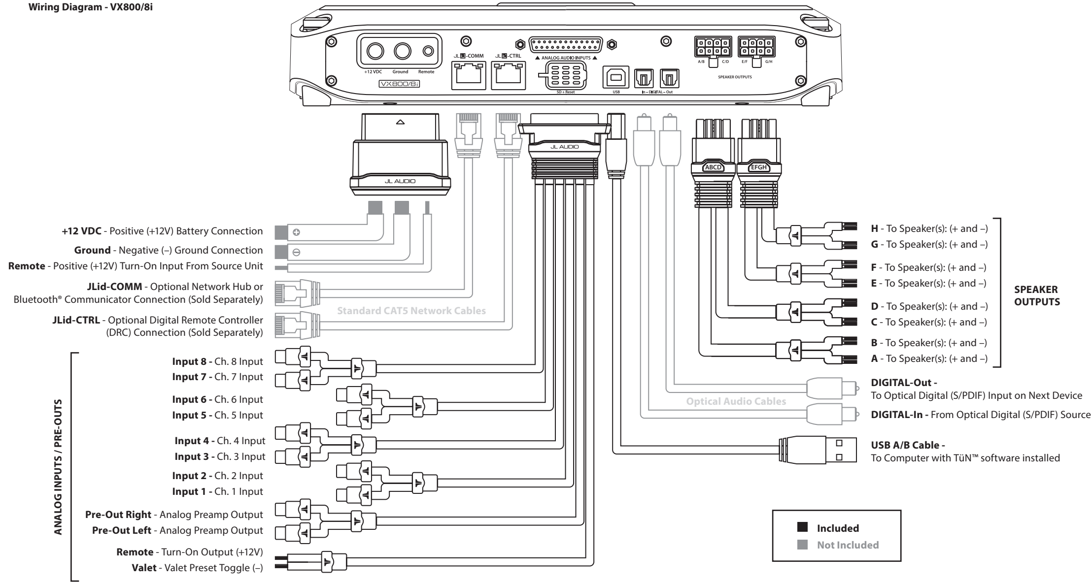
Wiring Diagram - VX800/8i
