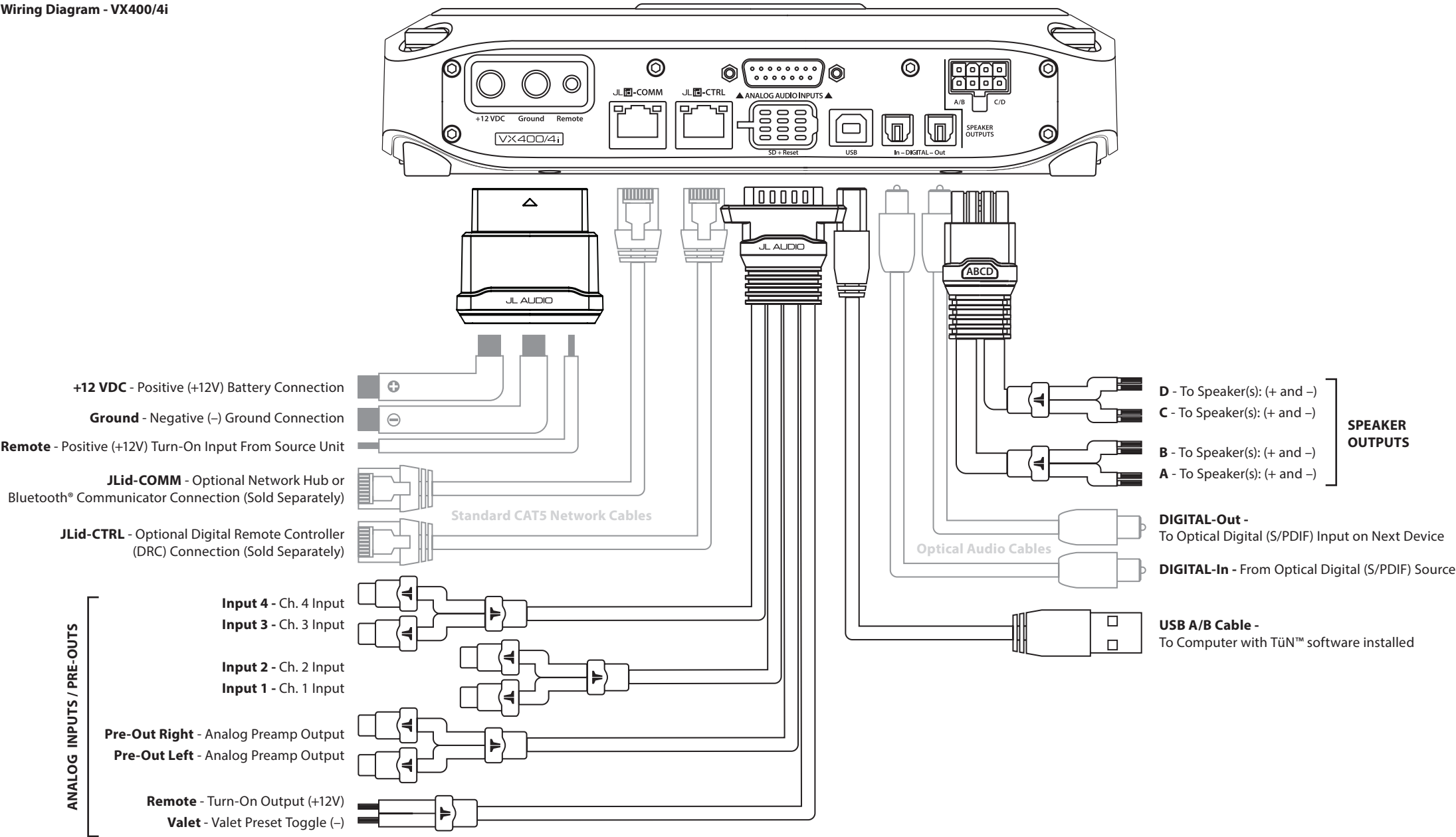
Wiring Diagram - VX400/4i
