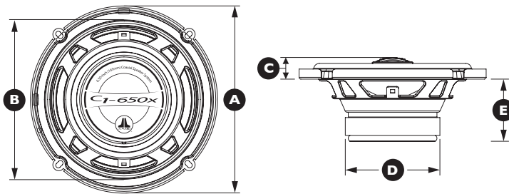
Coaxial Physical Dimensions
