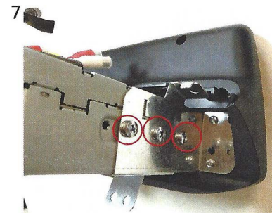
7 Insert the new radio unit as shown in the picture and fix it with 3 screws per side.
