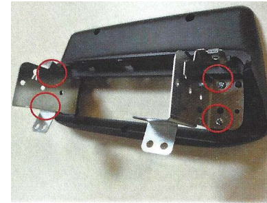
6 Fix the supplied brackets with the 2 screws per side as shown in the picture.
