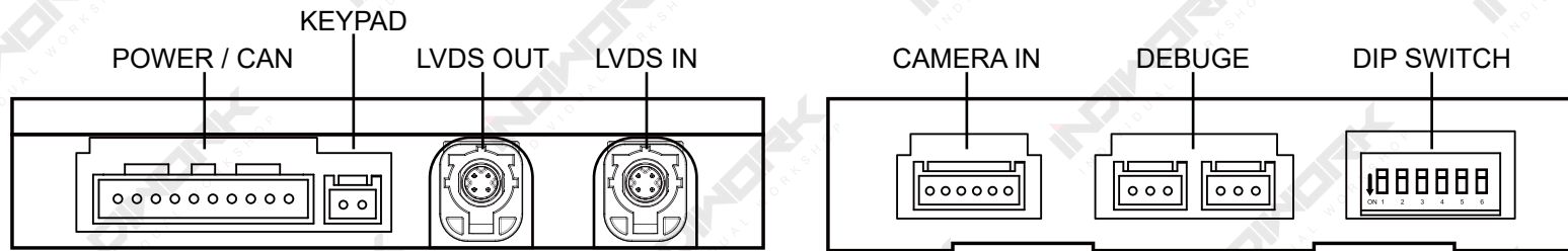
POWER/CAN CABLE
