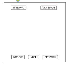
Multimedia System – Head Unit(in the glovebox)
