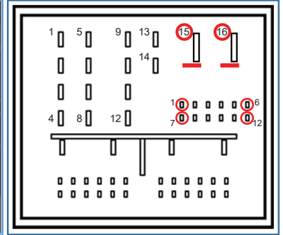
CAN wires Information
