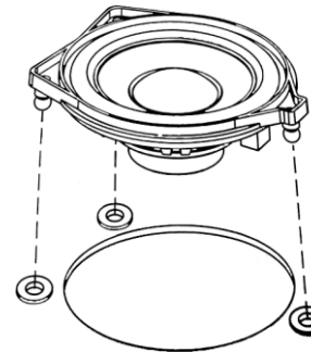
BL-MB100S (Two-way component speaker Pair)
