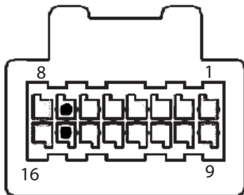
GMRVD Connector
