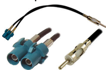
Double Fakra male to DIN male antenna adapter cable
